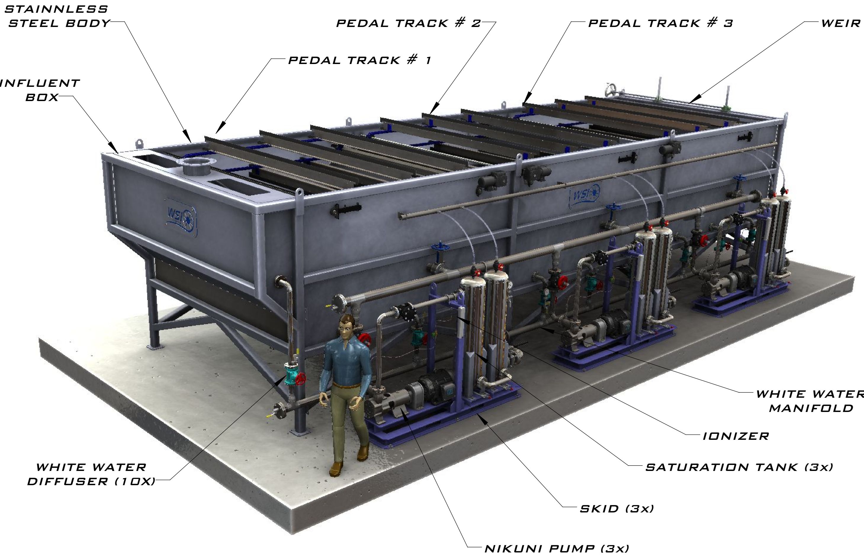
DISCHARGE SIDE
