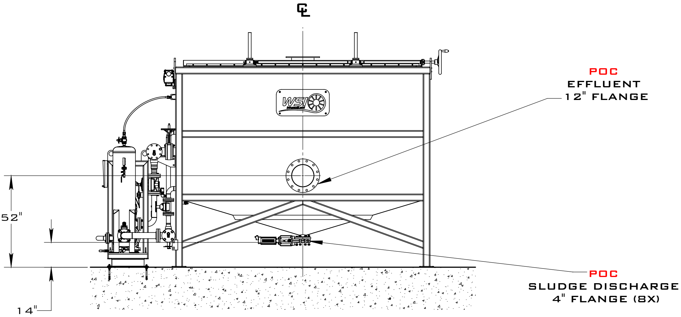
DISCHARGE SIDE
