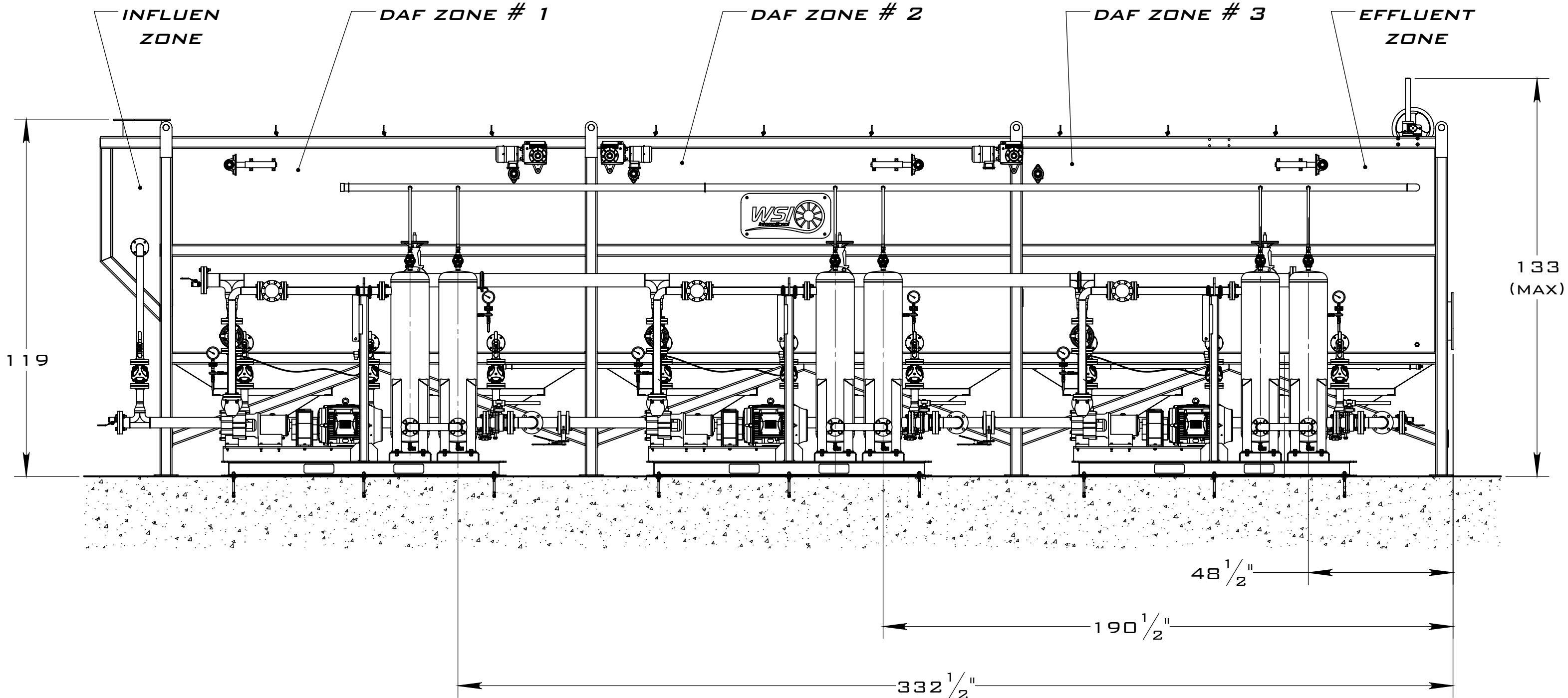
CONTROL SIDE
