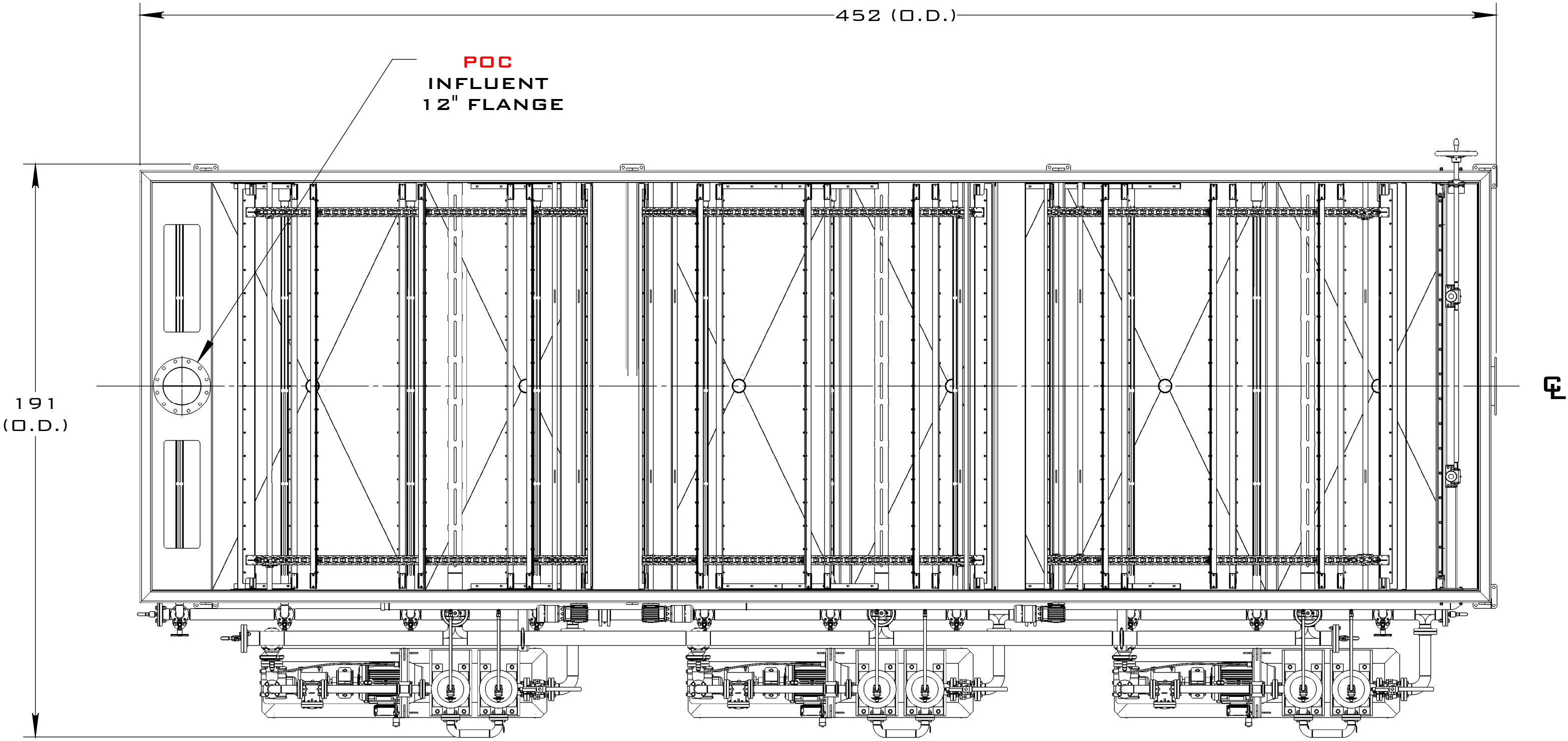
PLAN VIEW
